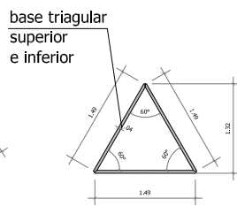
PLANTA BASE METALON (40x40mm)
